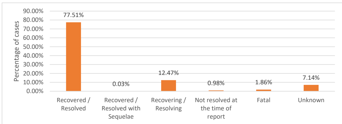
Figure 7. Case outcome
